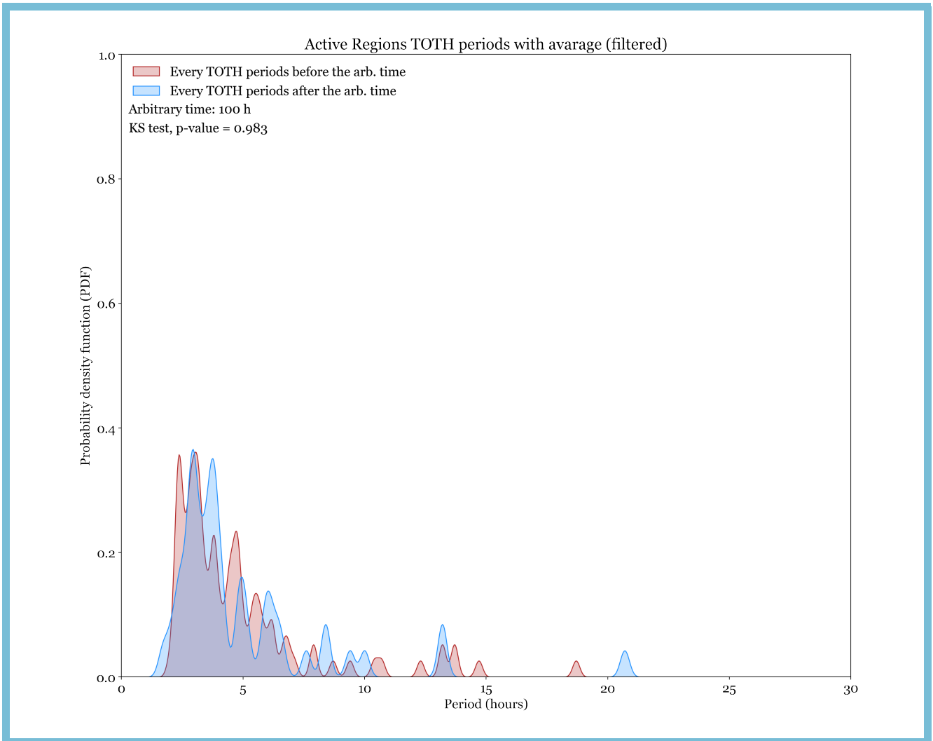
Figure 8. This figure is available as an animation which shows consecutive reference times of non-flaring T before/after the chosen reference time. Only small fluctuations are visible. The animation runs between arbitrary times 50 - 125 hours. The real-time duration of the animation is 2 seconds.
