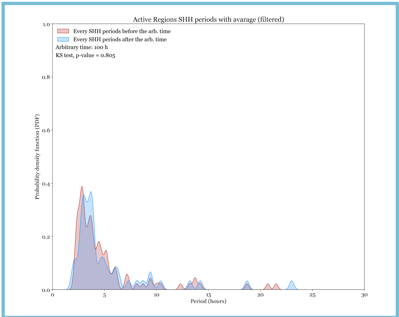
Figure 7. This figure is available as an animation which shows consecutive reference times of non-flaring SH before/after the chosen reference time. Only small fluctuations are visible. The animation runs between arbitrary times 45 - 130 hours. The real-time duration of the animation is 2 seconds.
