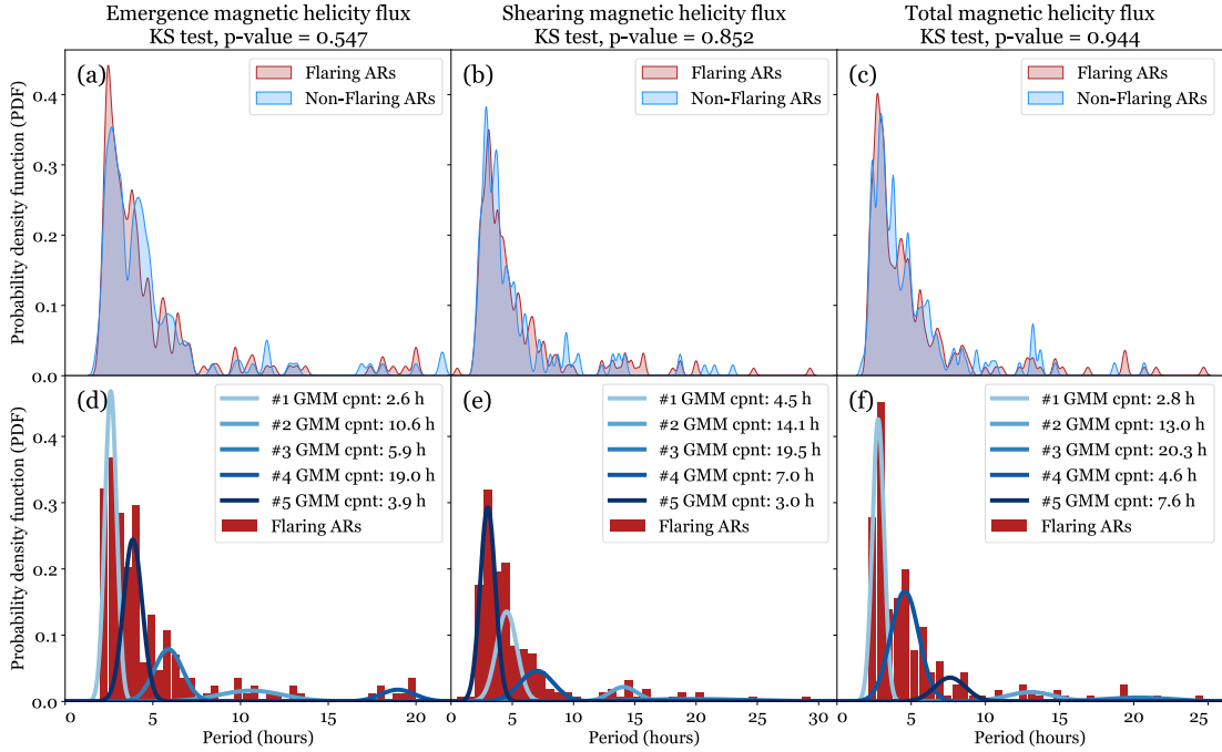
Figure 2. Top row: Normalized PDF of the WPS peaks of flaring (red) and non-flaring (blue) ARs for (a) emergence, (b) shearing, and (c) total helicity, using KDE. Note these results are for the smoothed time series. Using GMM, panels d-f show the corresponding distributions fitted to a set of Gaussian functions. The number of Gaussian components are set to 5. The 1/n -dependence refers to a power law, where n = 1, 2, 3, \dots is a positive integer, of the EM peaks of Gaussians is clearly visible in panel d.
