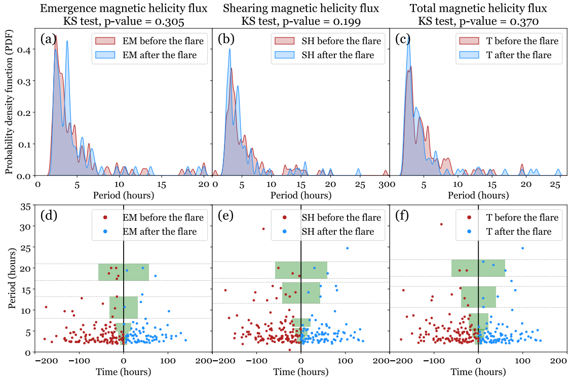
Figure 4. Panels a-c: Distribution of EM/SH/T peaks before (red) and after (blue) the flares. In the EM (a) case the most striking feature is that the short periods split into \sim 2.5 and \sim 4.5 hours after the flare occurred. Similar to the peaks of SH (b). Panels d-f: EM/SH/T periods of all flaring ARs. The black vertical line marks the reference time of the flares. The center of the green rectangles is given by the center of the Gaussian distributions fitted by the GMM method. The height of the rectangles corresponds to the FWHM value of the Gaussians fitted by the GMM method. The width of the green rectangles corresponds to 3 periods. The grey dashed lines are the boundaries of green rectangles, in case of the longer periods of EM/SH/T.
