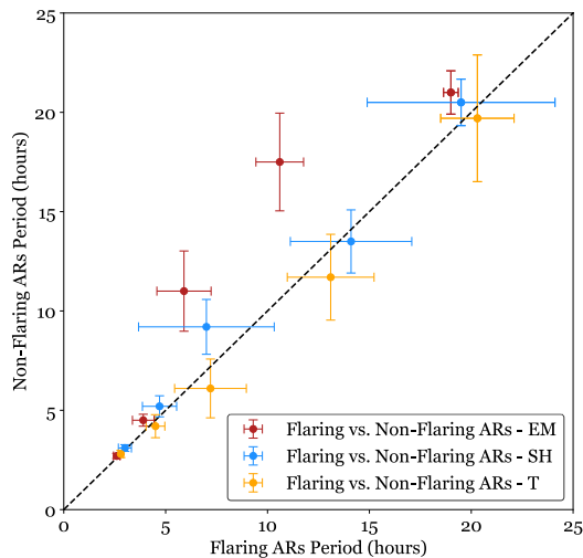
Figure 3. Correlation between the Gaussian-central periods of flaring and non-flaring ARs. The error bars are estimated with a bootstrapping method. The dashed black line shows the one-to-one correspondence between flaring and non-flaring periodicities. Only the EM periodicities are significantly above this line.
