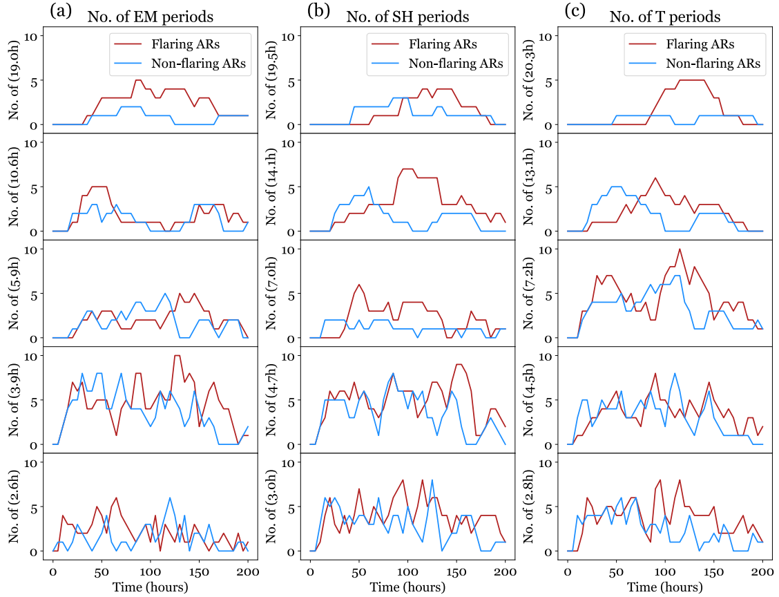
Figure 5. Number of (a) EM, (b) SH and (c) T oscillatory peak periods in flaring and non-flaring ARs. The blue/red lines correspond to non-flaring/flaring ARs. Long periods ( \sim 20 hour) appear in the oscillatory peaks of the WPS of the T and EM fluxes of flaring ARs, which seem to be linked to flare/CME eruptions.
