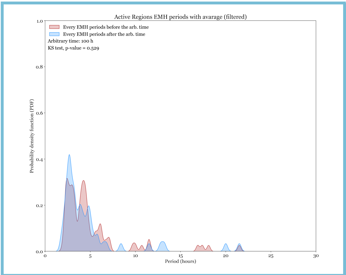
Figure 6. This figure is available as an animation which shows consecutive reference times of non-flaring EM before/after the chosen reference time. Only small fluctuations are visible. The animation runs between arbitrary times 40 - 140 hours. The real-time duration of the animation is 2 seconds.
